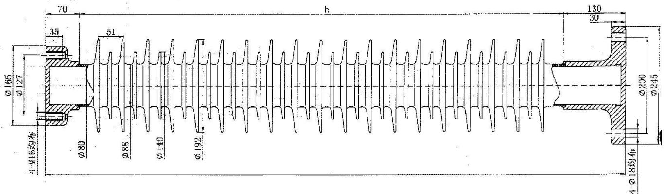
Fig.18 252kv composite post insulator
