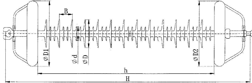
Fig.10 330KV AC composite
