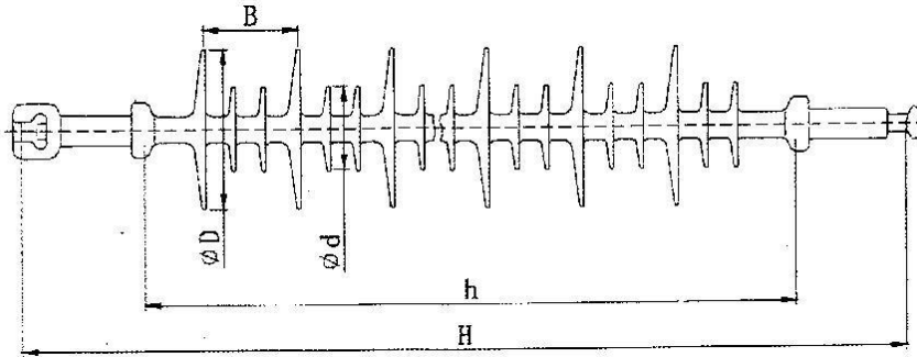
Fig.7 35KV~66KV AC composite insulator General
