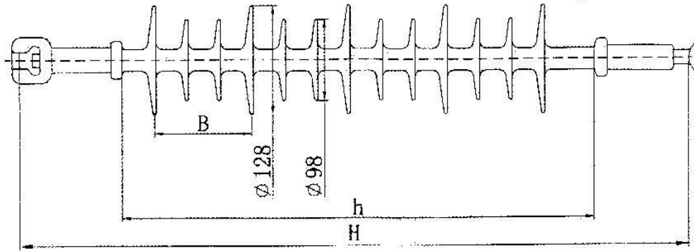
Fig.21 Composite insulator for traction transformer substation
