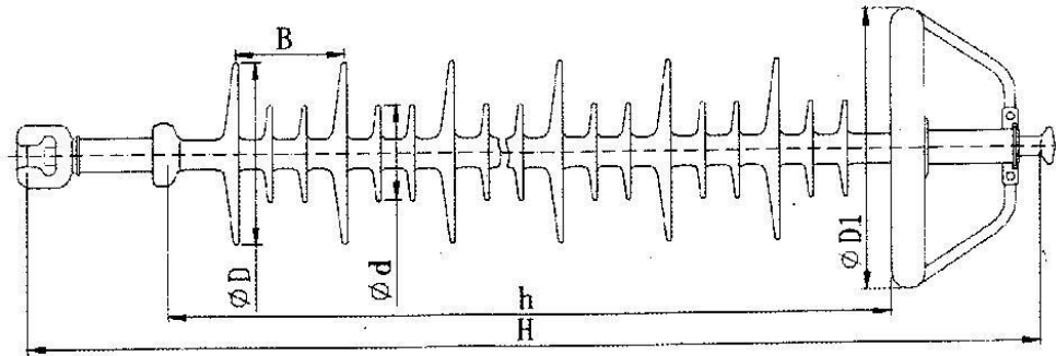
Fig.8 110KV composite insulator General
