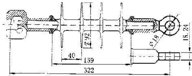
Fig.4 10KV composite insulator (W, D coupling)
